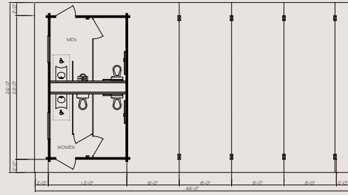
GAR2648 26' x 48' with 22' x 12' Enclosed
