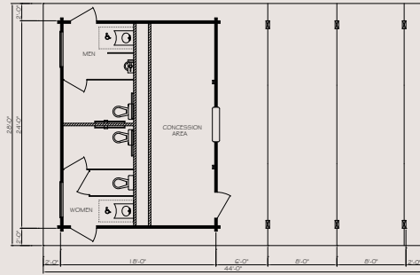
GAR2844 28' x 44' with 24' x 18' Enclosed
