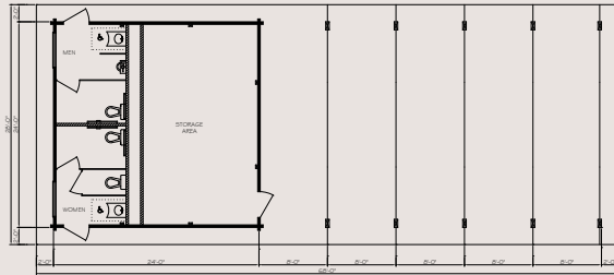
GAR2868 28' x 68' with 24' x 24' Enclosed
