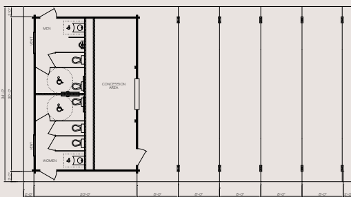
GAR3464 34' x 64' with 30' x 20' Enclosed
