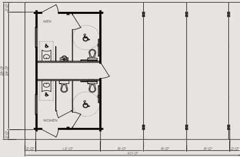
GAR2840 28' x 40' with 24' x 12' Enclosed
