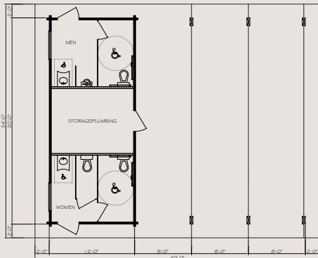
GAR3440 34' x 40' with 30' x 12' Enclosed
