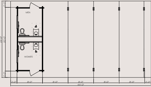
GAR2444 24' x 44' with 20' x 8' Enclosed
