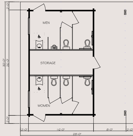
GAR3028 30' x 28' with 26' x 16' Enclosed
