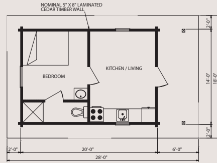
Northland: 14' x 20', 280 sq. ft.
