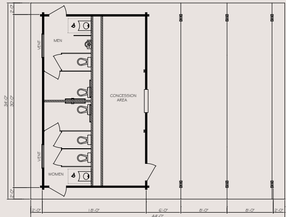
GAR3444 34' x 44' with 30' x 18' Enclosed
